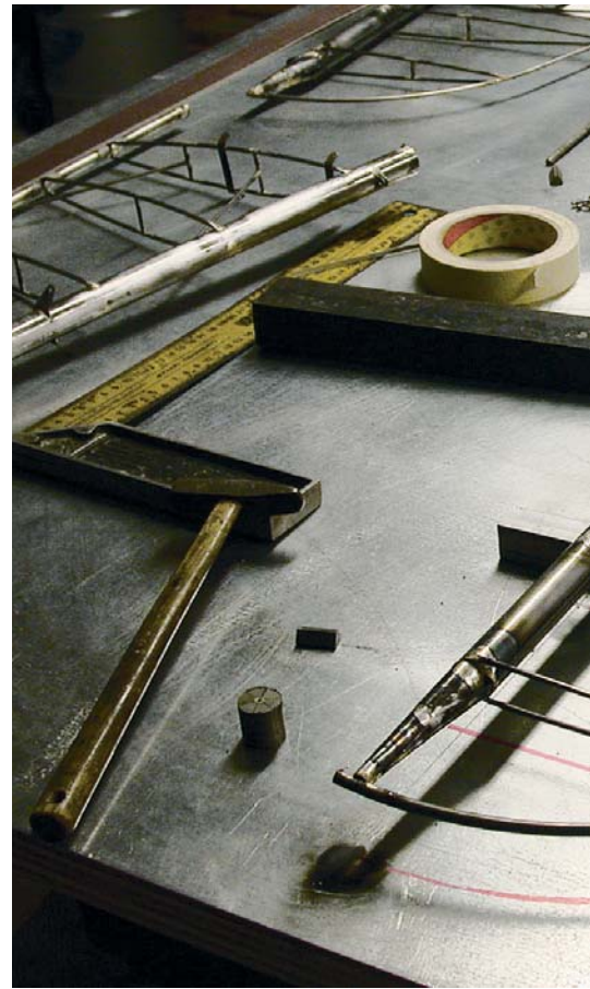
Above and below: construction of the tailplane with steel tube
